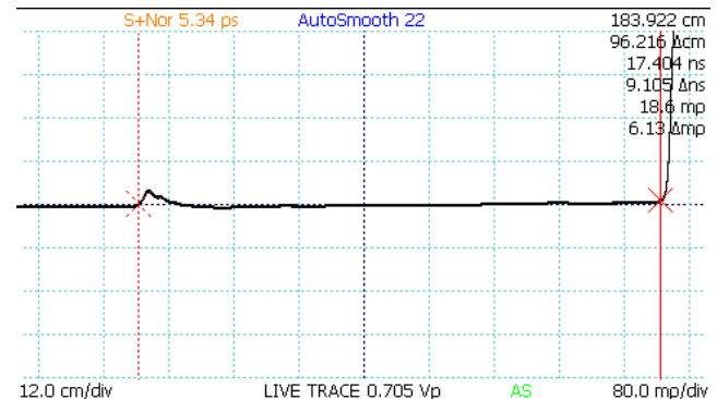
Figure 3: Measurement of distance between soft faults.
