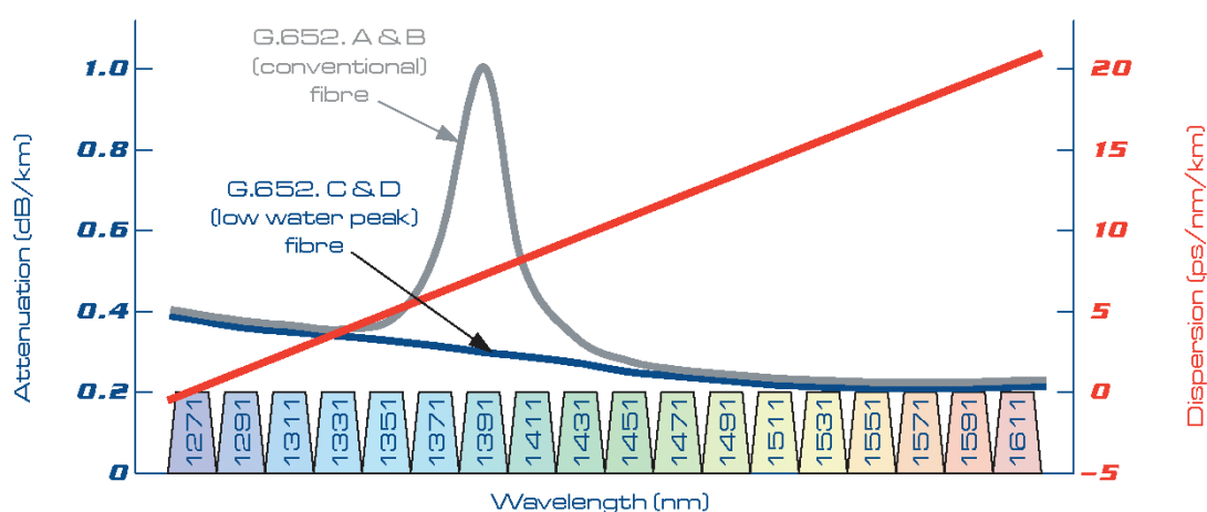
ITU-T G.694.2 - CWDM Wavelength Grid
