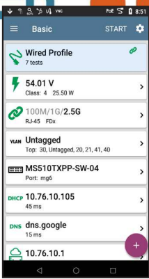
NBASE-T switch network with VLAN and 802.1x authentication
